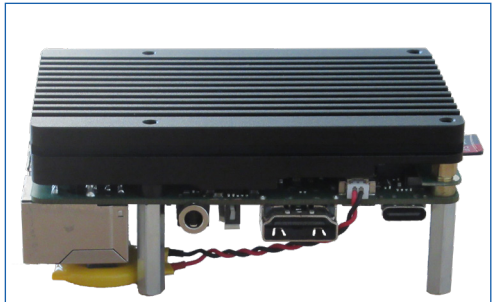
Rock Pi4 internal connections and SD slot
